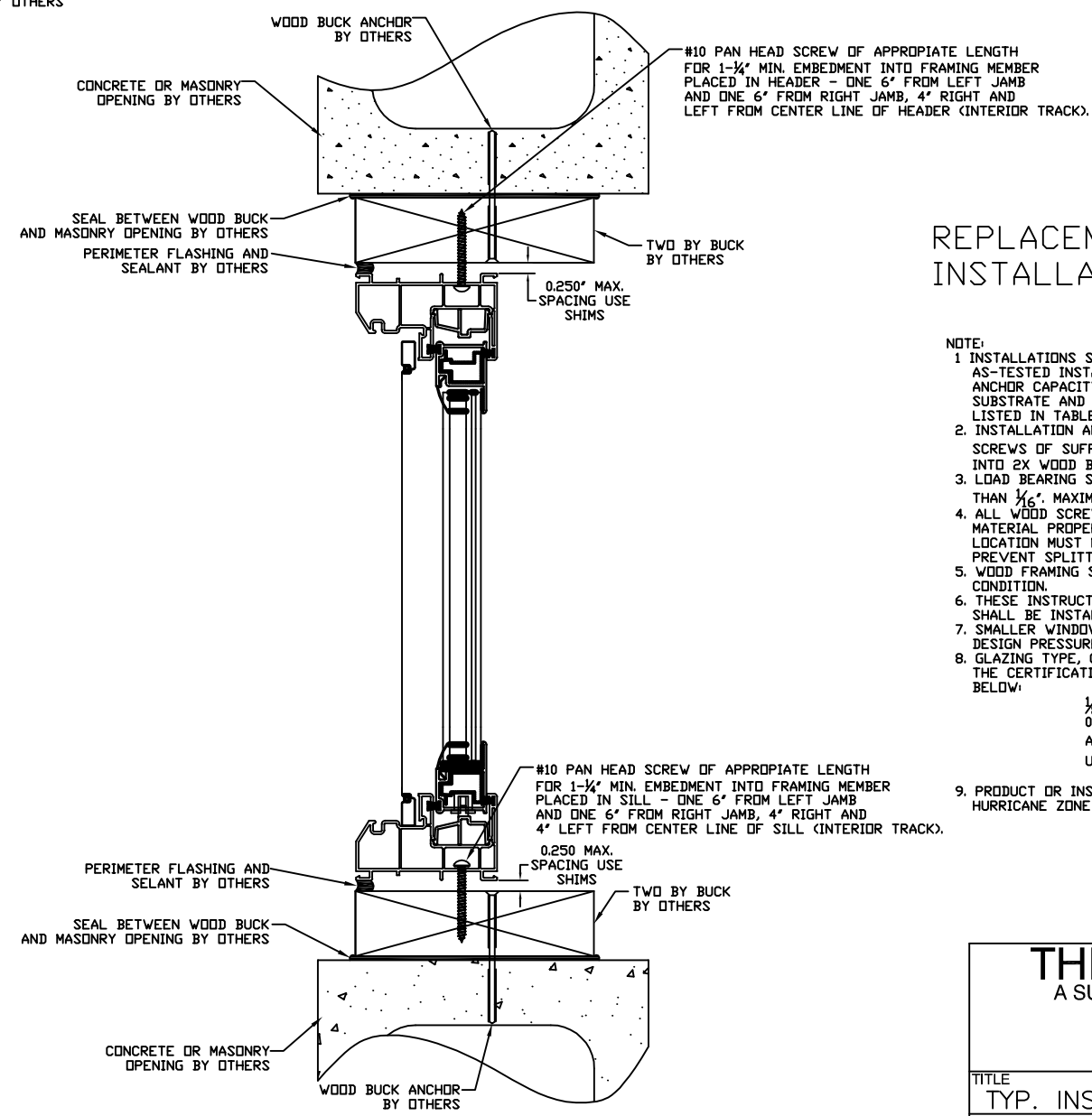
VERTICAL CROSS SECTION - WINDOW IN WALL
