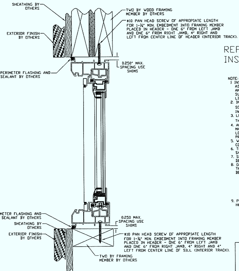
VERTICAL CROSS SECTION - WINDOW IN WALL
